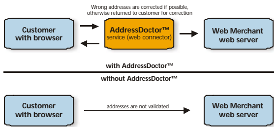
Online shops with and without the Web Connector
